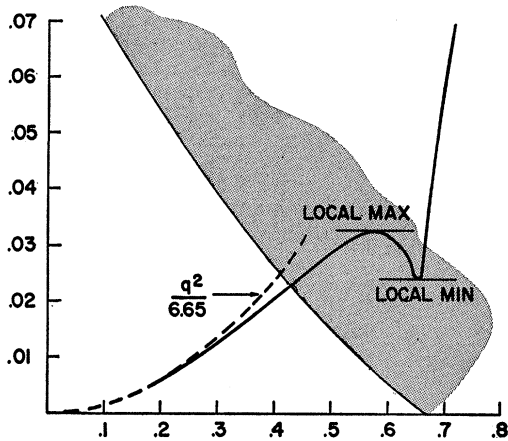
FIG. 3. Same as Fig. 2, but \Delta = 0.9 for comparison.
